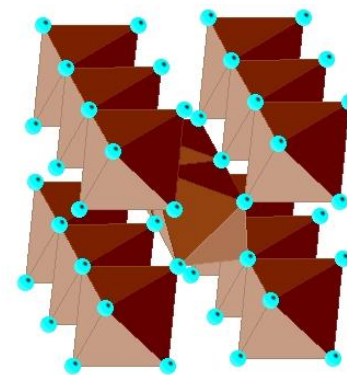
\text{MgH}_2
